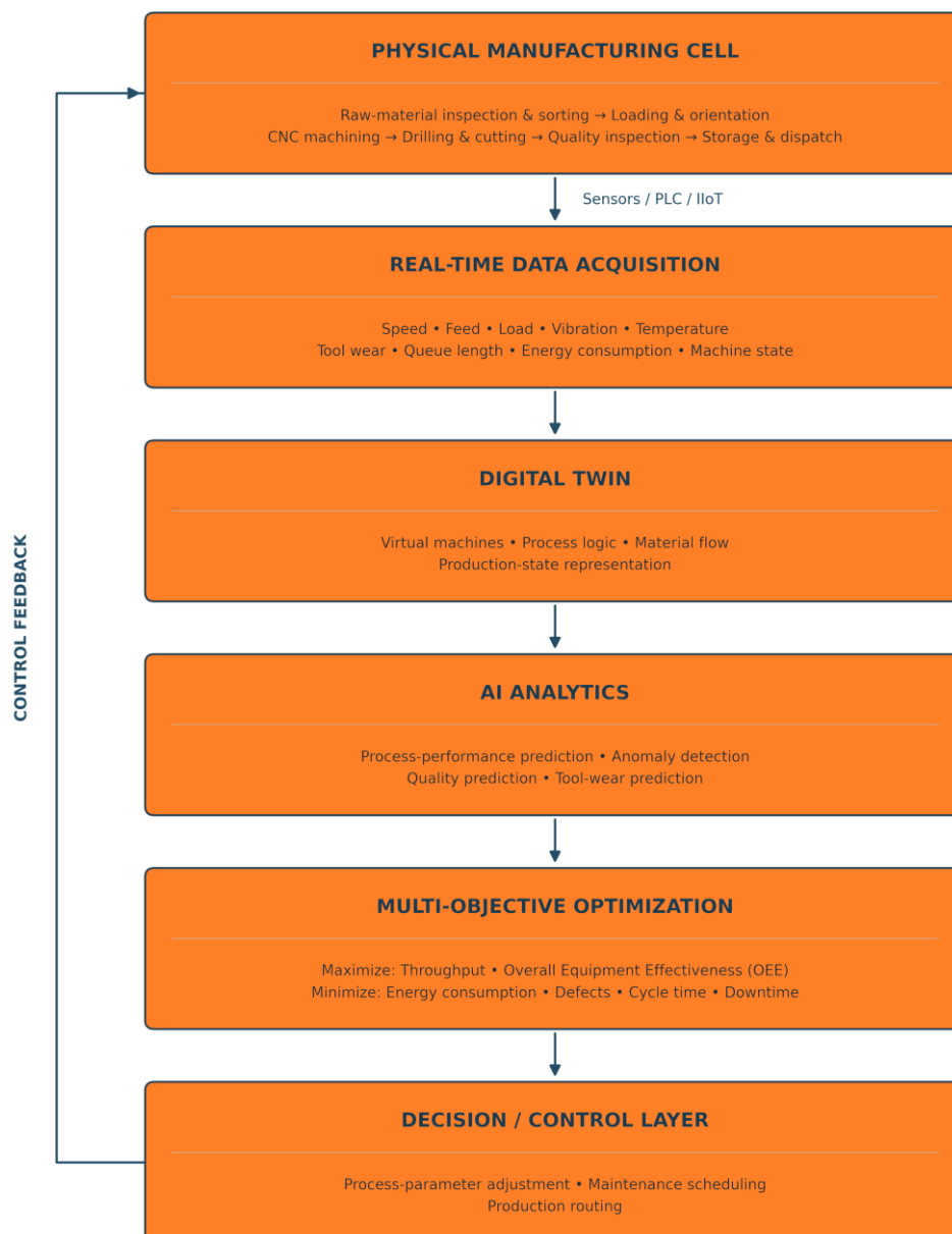
Figure 1. Digital Twin–AI architecture for the proposed mechanical manufacturing system
